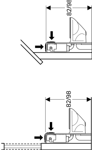
← LOW-HEIGHT SITUATIONS Solution for low-height installation with element heights 82 cm, choose either Omega or Alpha. For a height of 98 cm go for Omega.
